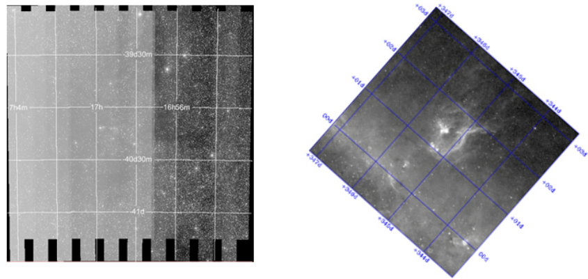
Figure 1. Original 2MASS and MSX images
