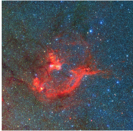
Figure 2. Final 3-color mosaic: MSX A-band is red, 2MASS K-band is green, and 2MASS J-band is blue.
